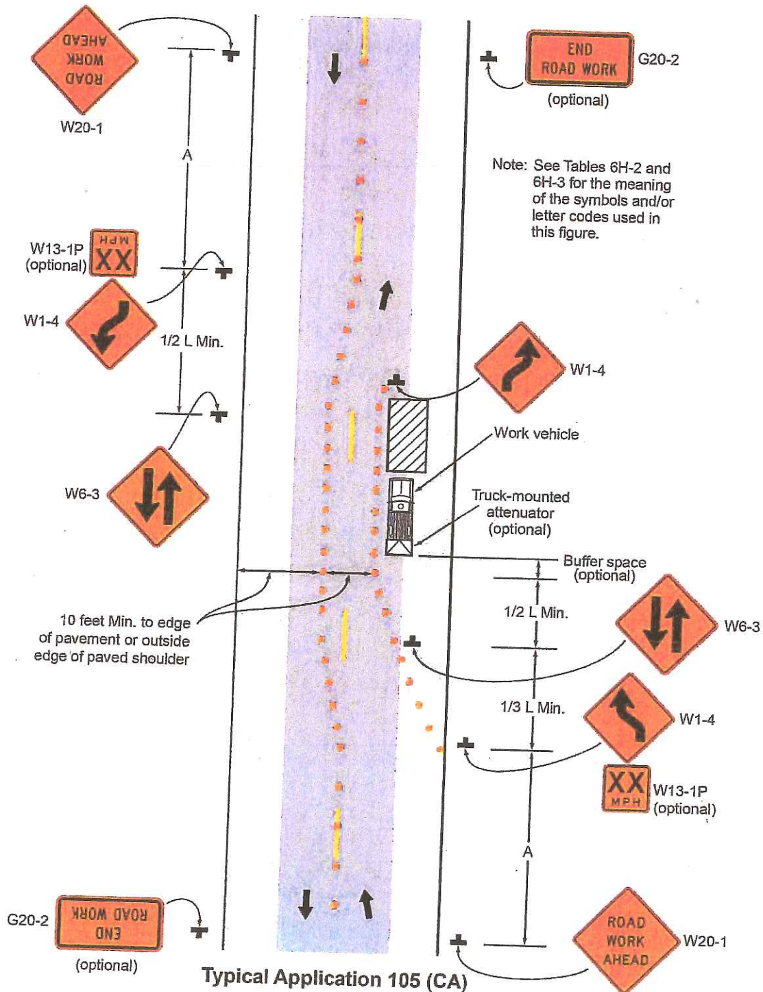
Figure 6H-105 (CA). Lane Shift on Road With Low Traffic Volumes (TA-105 (CA))
